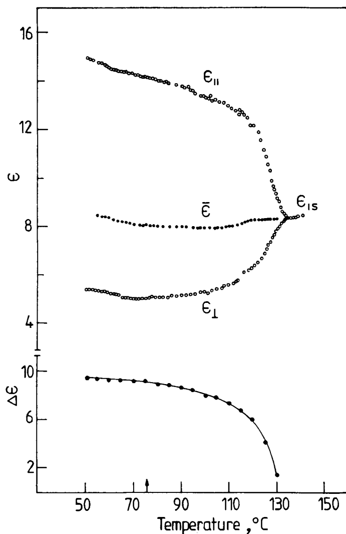
FIGURE 6 The low frequency principal dielectric constants and the dielectric anisotropy ( \Delta\epsilon = \epsilon_{||} - \epsilon_{\perp} ) at 1592 Hz of the 60% 4 PCPP mixture as functions of temperature. The vertical arrow on the temperature axis indicates the nematic-smectic transition point.
